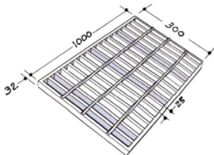
STEEL GRATING COVER 300MM X 1000MM WITH HOT DIP GALVANIZE AND TWISTED ROD ( TRAFFIC TYPE)
